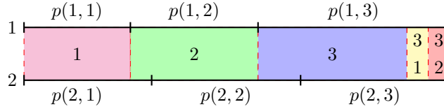
Figure 1: The graphical representation of the greedy Markovian coupling on three states starting from (1, 2) . Here, (28) follows from Assumption 1, which guarantees the “overlap”, or leftover probability with which the process does not couple.
