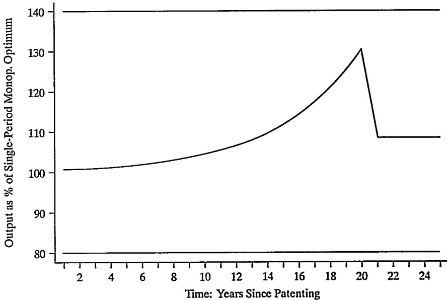
FIGURE 2: PATENTEE'S OPTIMAL OUTPUT OVER TIME GIVEN TRADEMARK LEVERAGE, AS PERCENT OF SINGLE-PERIOD MONOPOLY OPTIMUM
